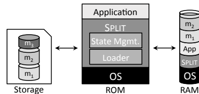
Figure 2. Functionality with a high memory footprint is split into modules and stored on the external storage. When needed, these are loaded, prepared, and executed.
