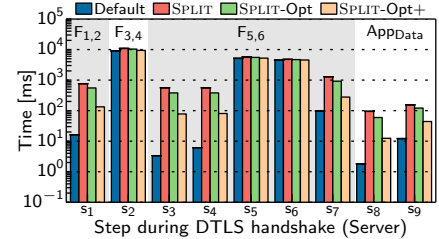
(c) Default vs. SPLIT Server (default counterpart). Annotations correspond to DTLS flights.
