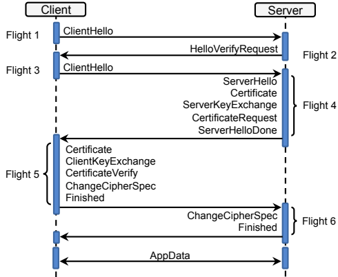
Figure 3. We separate DTLS messages into modules (individual messages). The granularity is tunable and protocol determinism allows for mitigating latency overheads.
