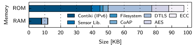
Figure 1. Memory requirements for a typical IoT stack.
