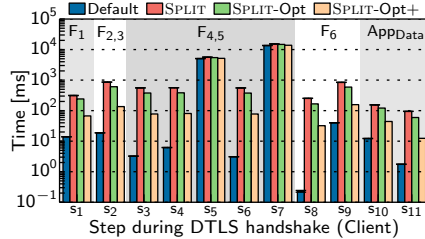
(b) Default vs. SPLIT Client (default counterpart). Annotations correspond to DTLS flights.
